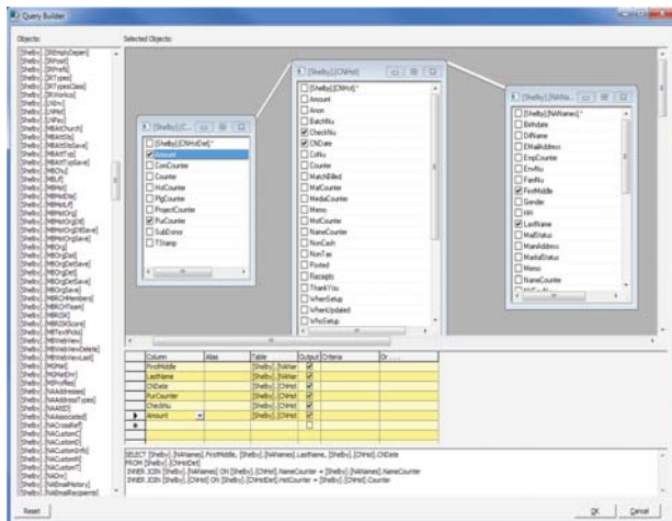
The graphical Query Builder makes it easy to see field and table relationships to help build complex SQL statements.
